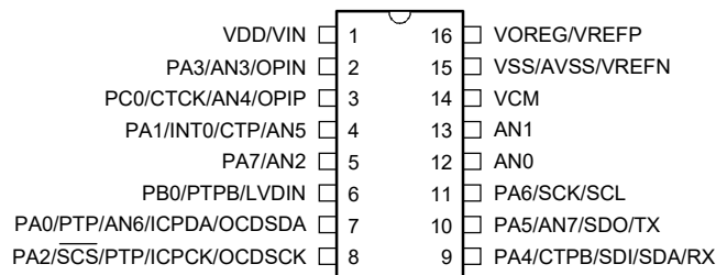
BH66F5242/BH66V5242 16 NSOP-A/SSOP-A
