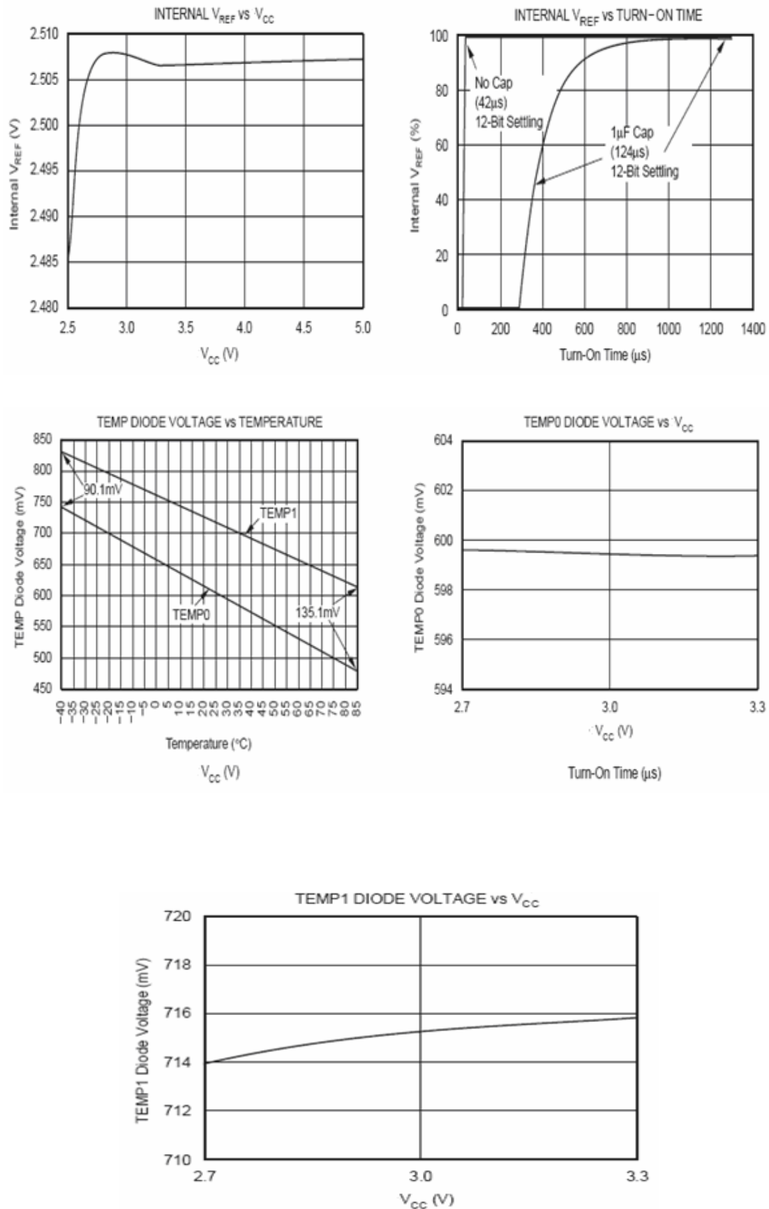
Figure 3. Typical Characteristics
